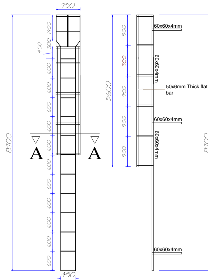
Ladder Details
