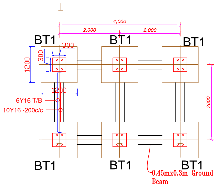
FOUNDATION DETAILS
