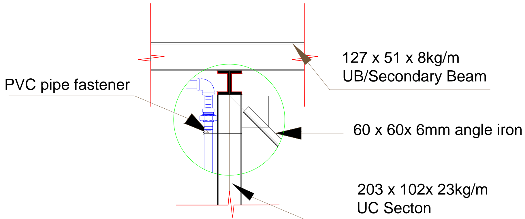
DETAIL C
