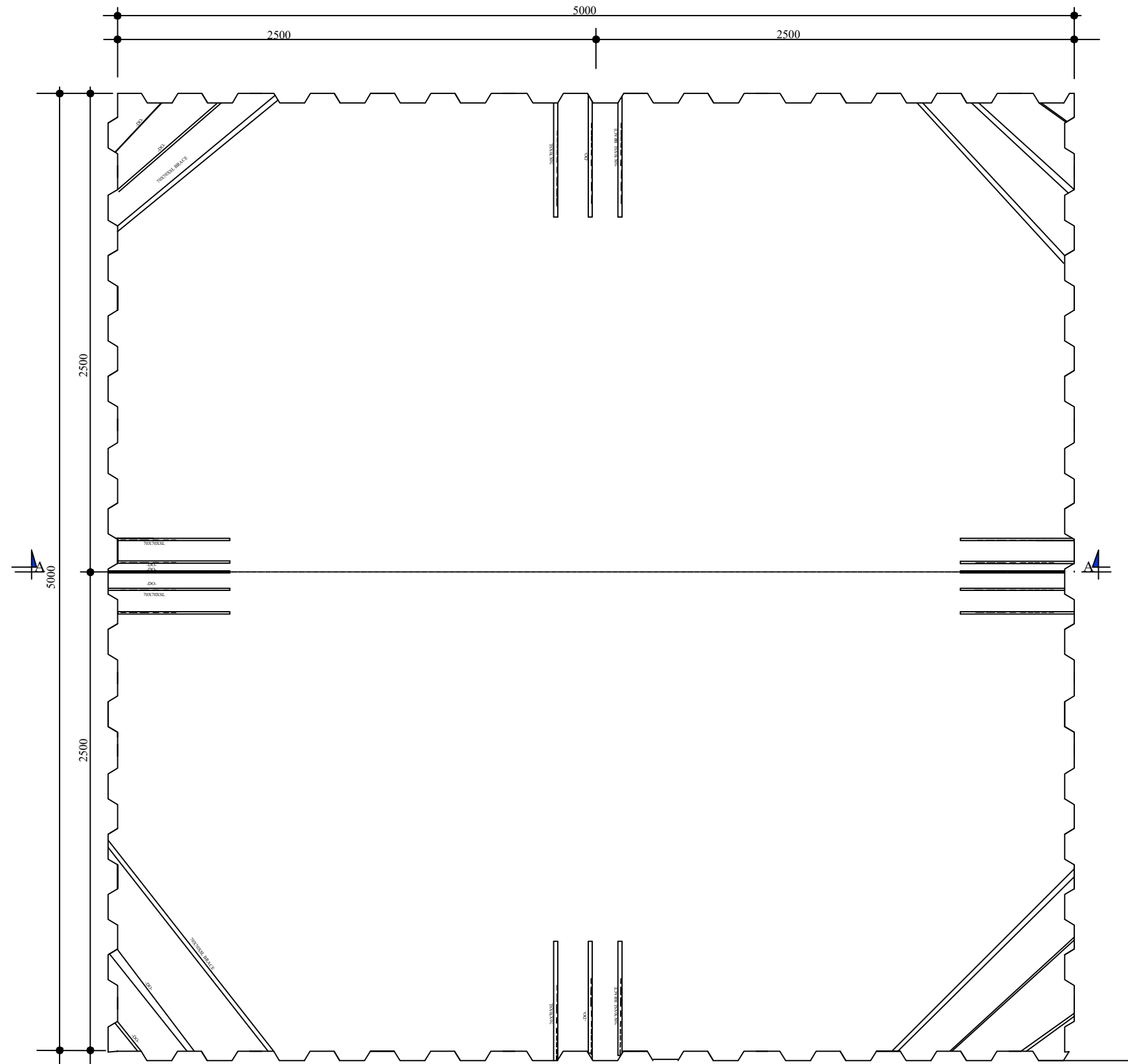
PLAN SHOWING INTERNAL BRACES (5m X 5m X 2.4m)
