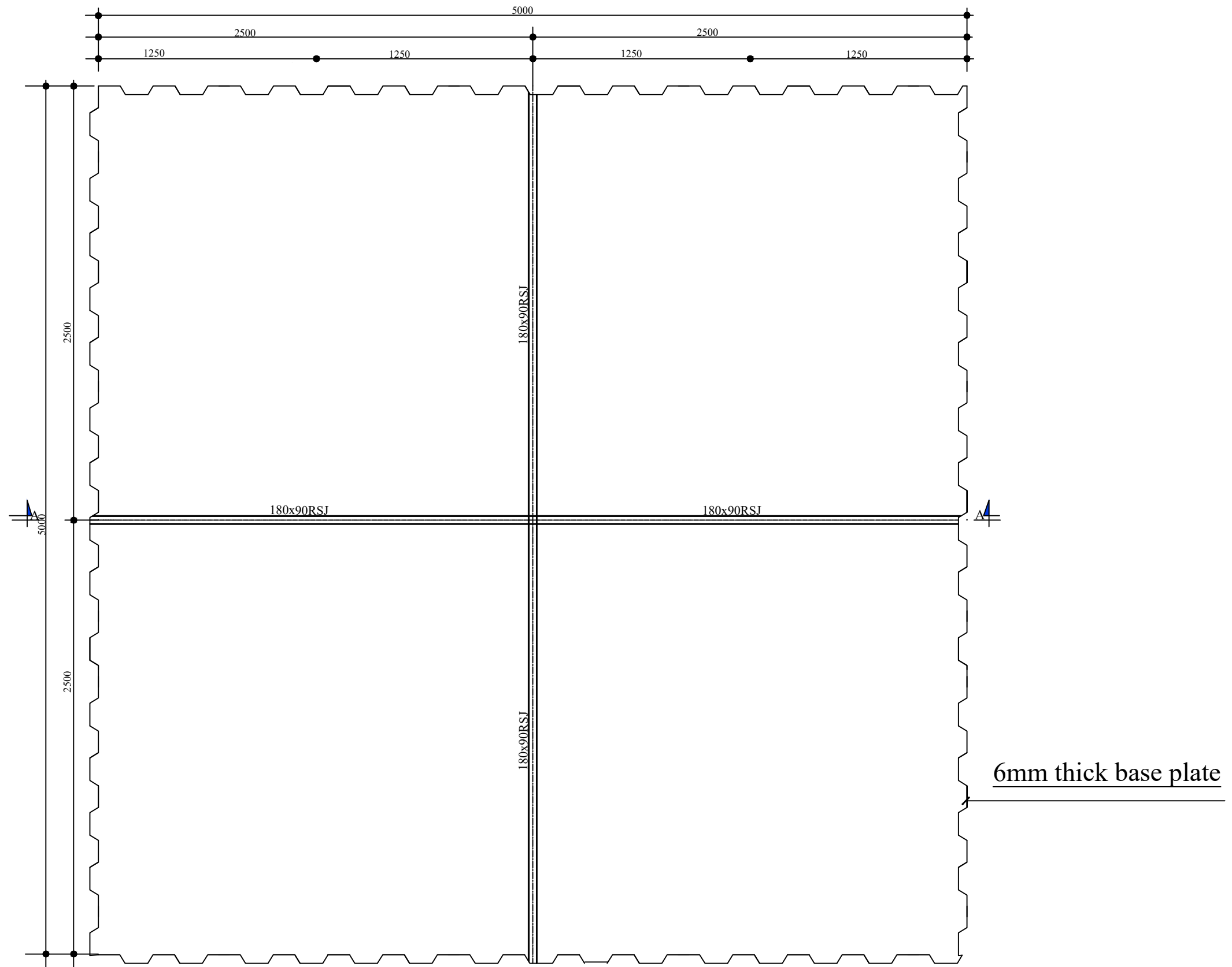
PLAN OF(GROUND TANK),50,000 LITRES (5m X 5m X 2.4m) INTERNAL BRACES STRUCTURES
