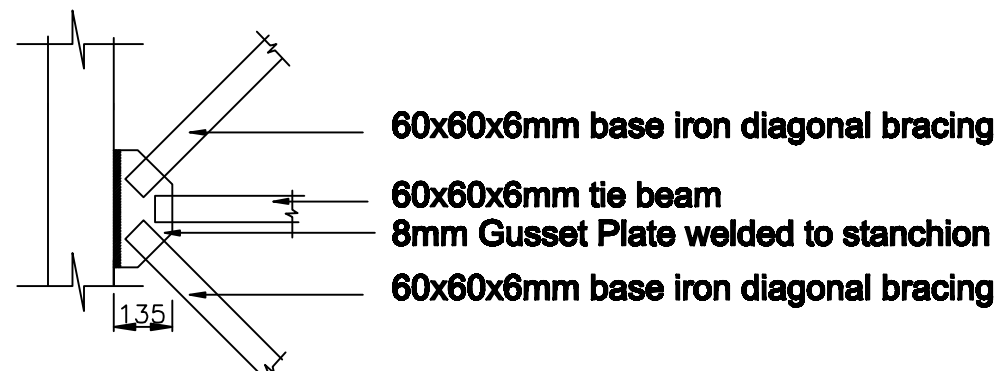
DETAIL-X
