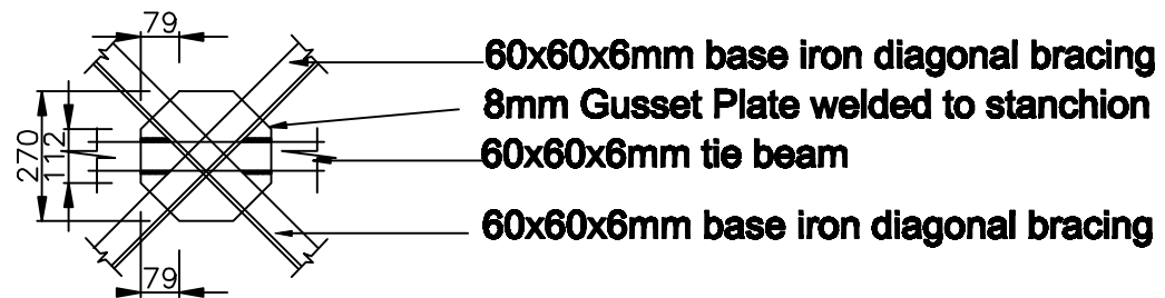
DETAIL-Y
